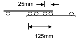
Reinforcing Rib Mesh Side Lap Save
